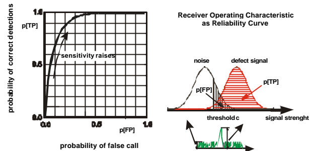
Figure 3: Characteristic of one NDT-System by an ROC curve
