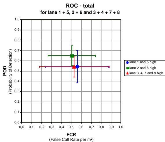
Figure 18: ROC-total
